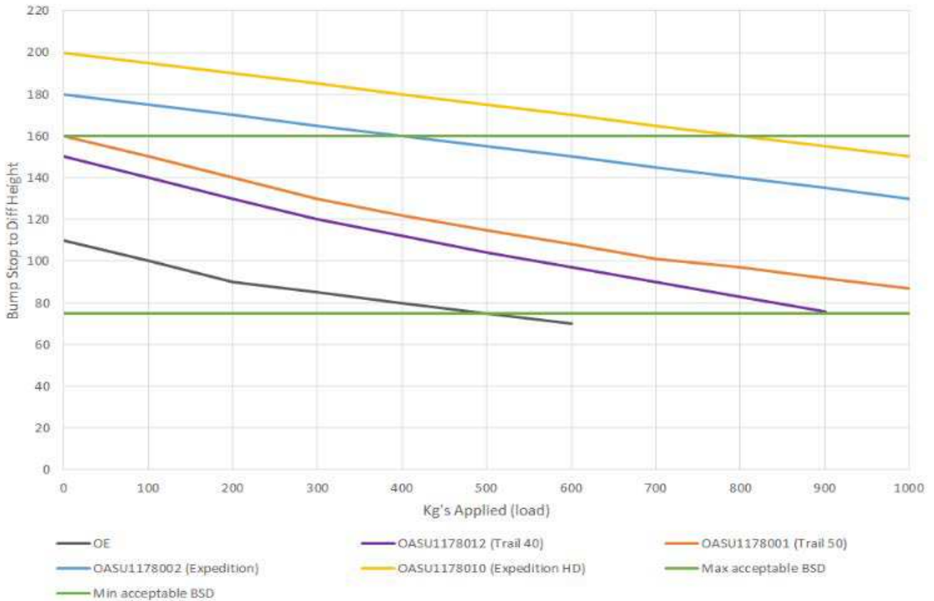
Toyota Landcruiser 79 Series Leaf Spring Deflection
