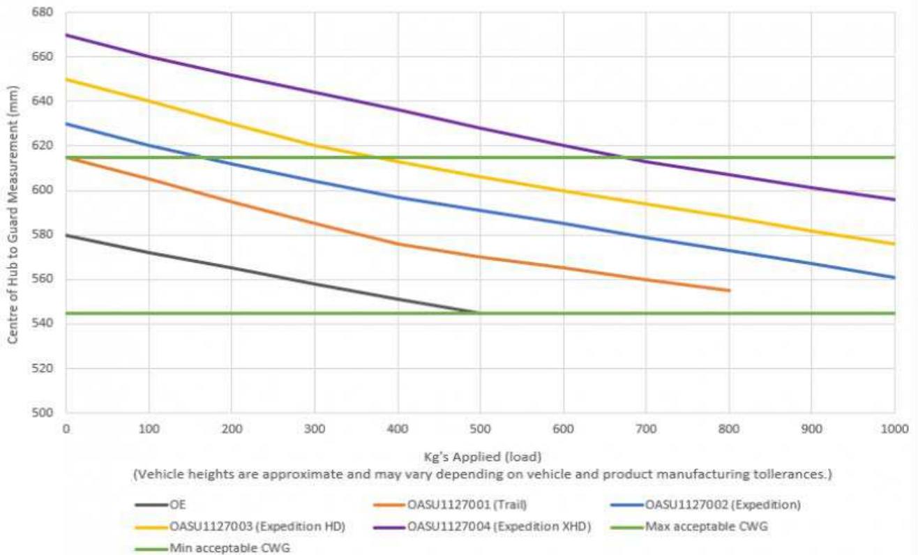
Volkswagen Amarok Leaf Spring Deflection
