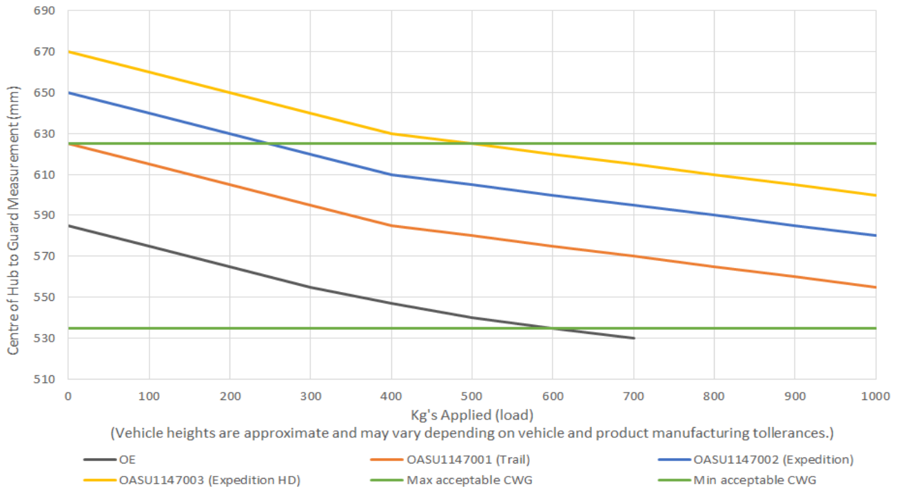
Mitsubishi Triton ML/MN Leaf Spring Deflection (Factory flared models)
