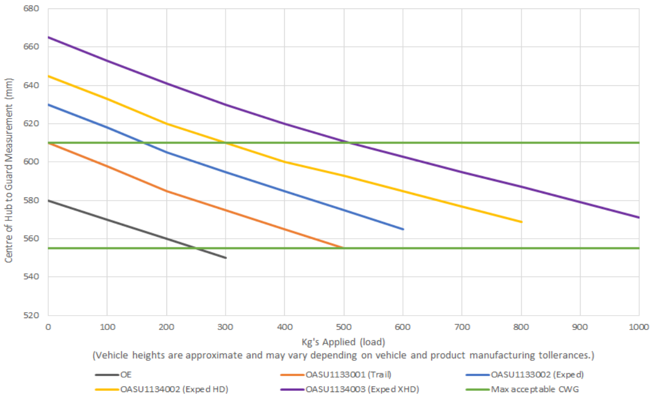
Holden Colorado RG Leaf Spring Deflection
