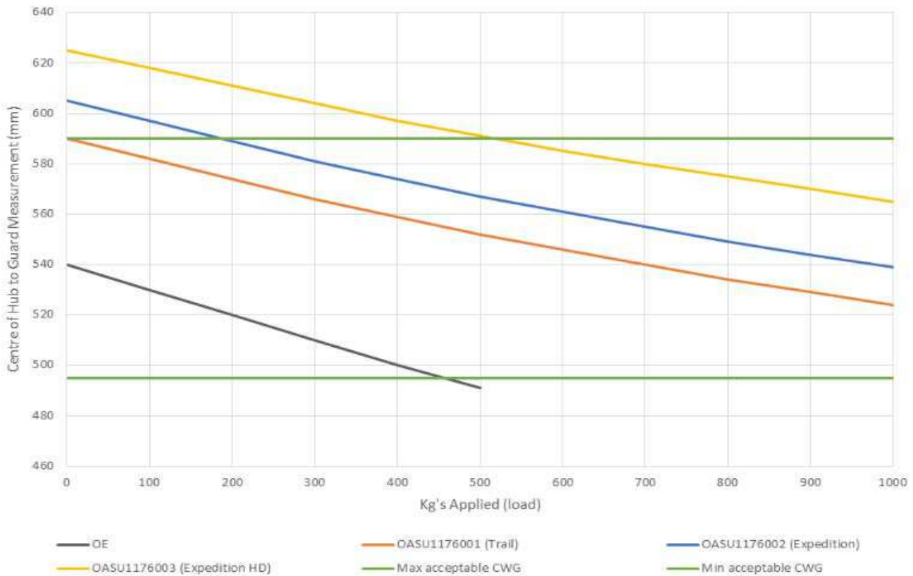
Toyota Landcruiser 76 Series Leaf Spring Deflection
