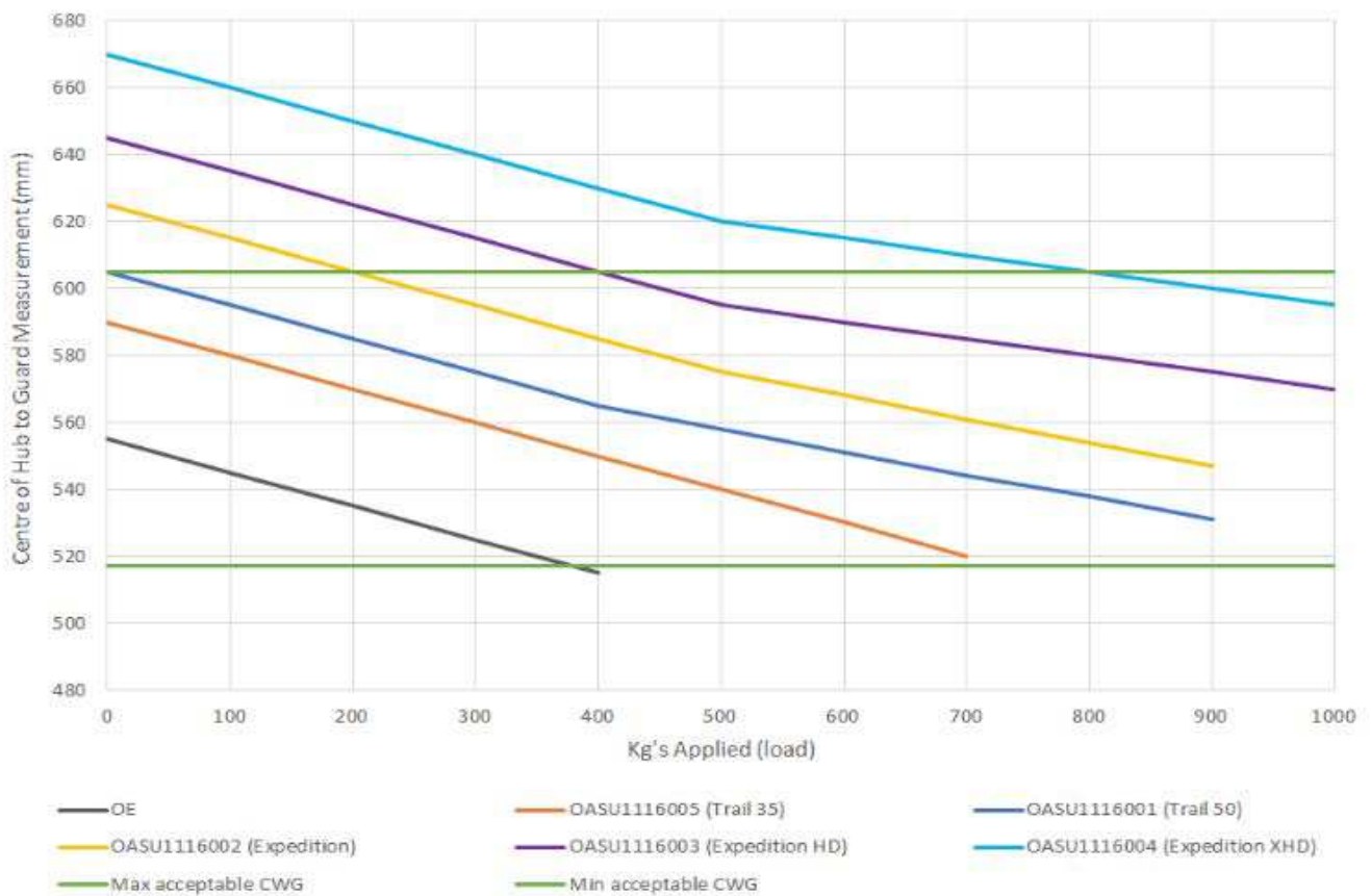
Toyota Hilux Gen 8 Leaf Spring Deflection
