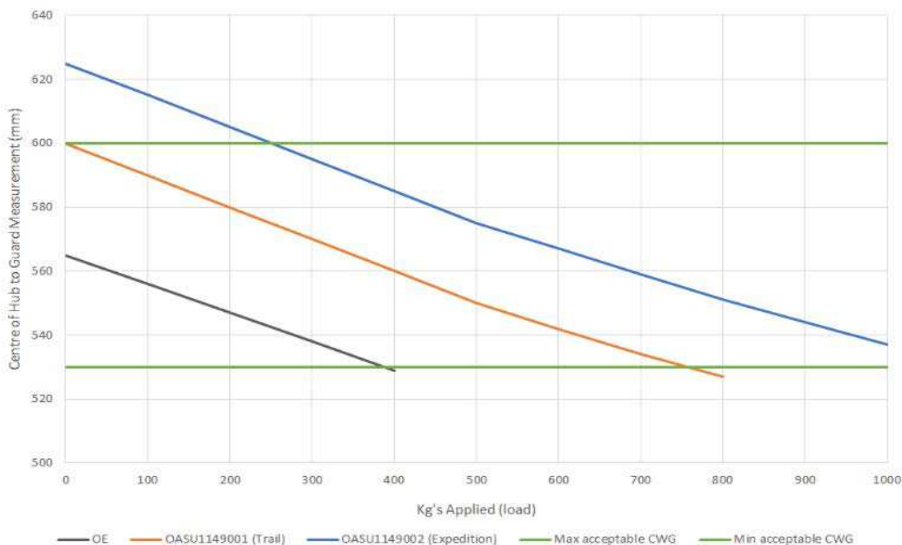
Ford Ranger PJ-PK / Mazda BT-50 Leaf Spring Deflection
