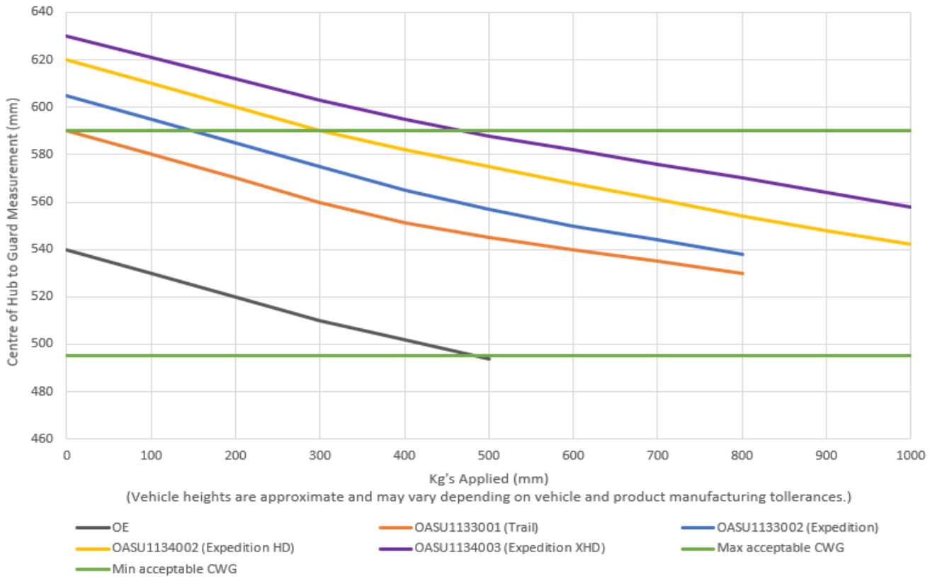
Isuzu D-Max 2012+ Leaf Spring Deflection
