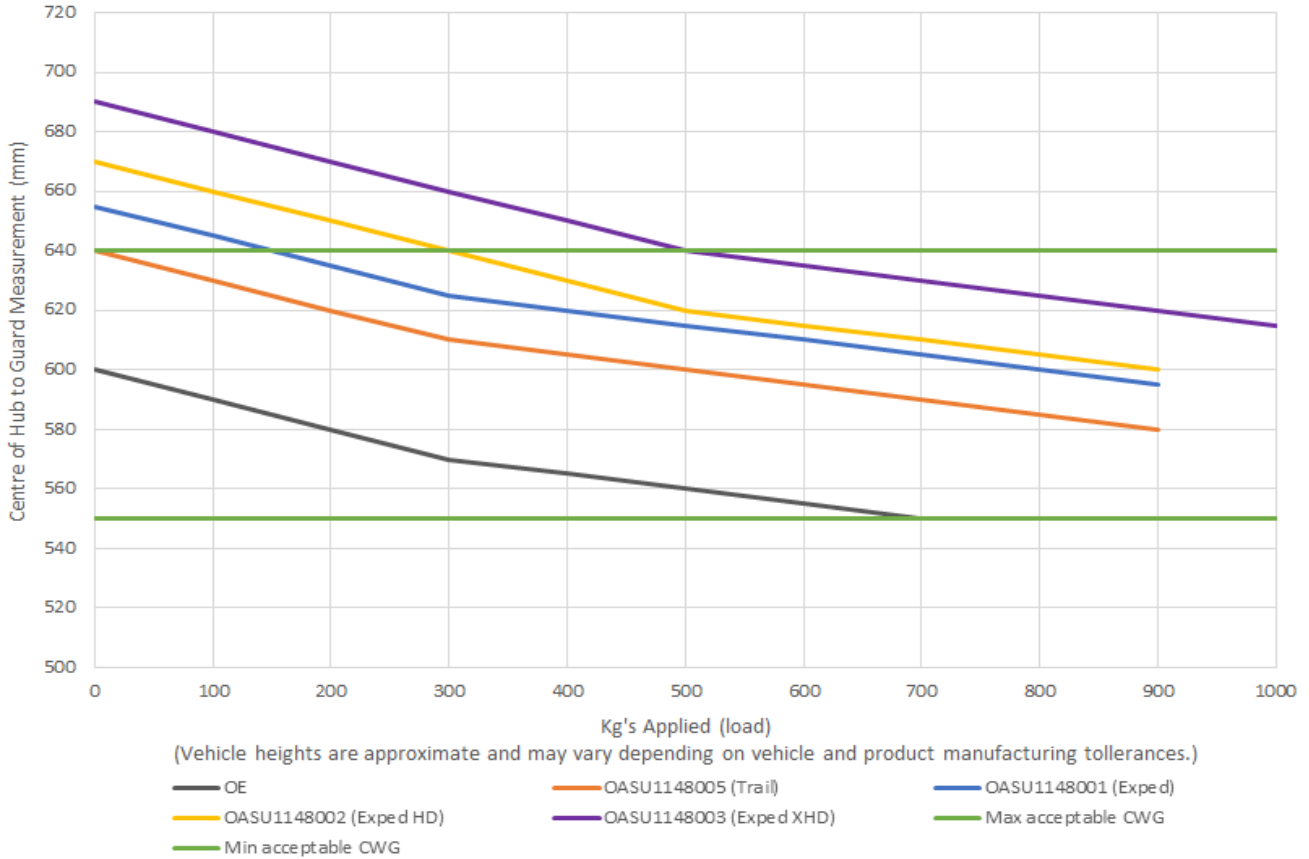
Ford Ranger PX-PXII / Mazda BT-50 Leaf Spring Deflection
