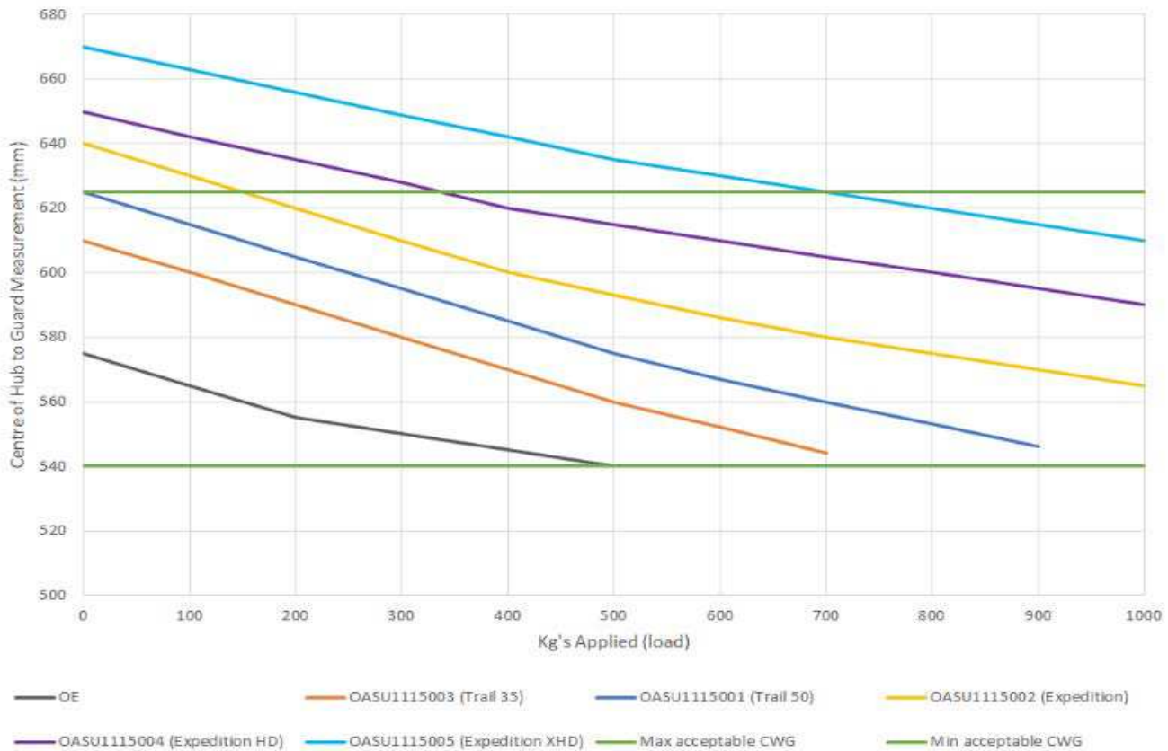
Toyota Hilux 150 Series Leaf Spring Deflection
