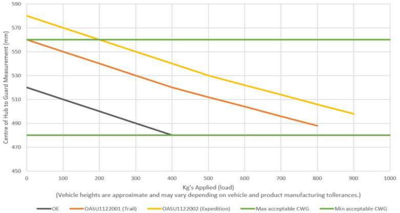
Nissan Navara D22 Leaf Spring Deflection
