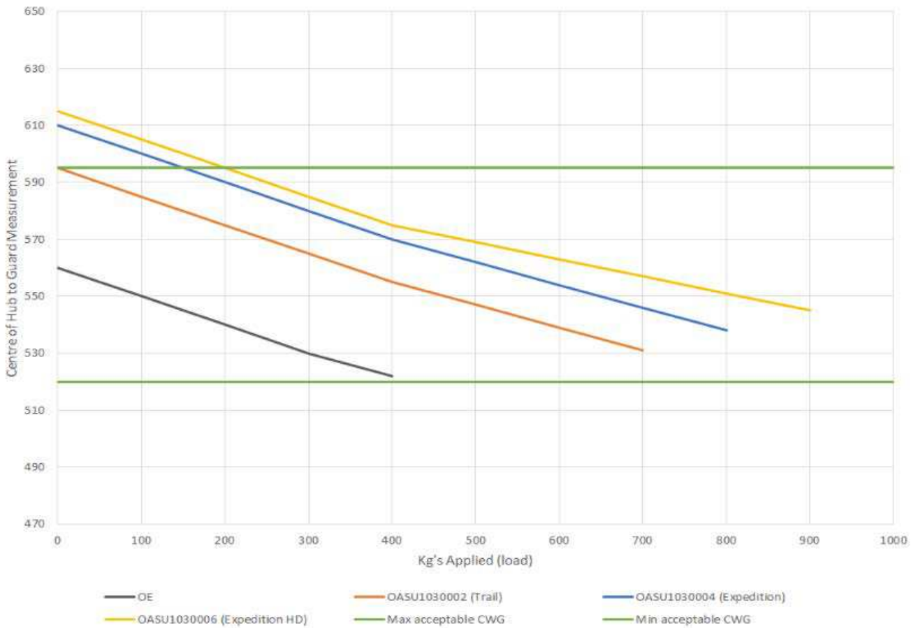
Nissan Navara NP300 Leaf Spring Deflection
