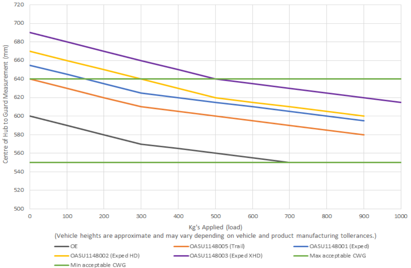
Ford Ranger PX-PXII / Mazda BT-50 Leaf Spring Deflection
