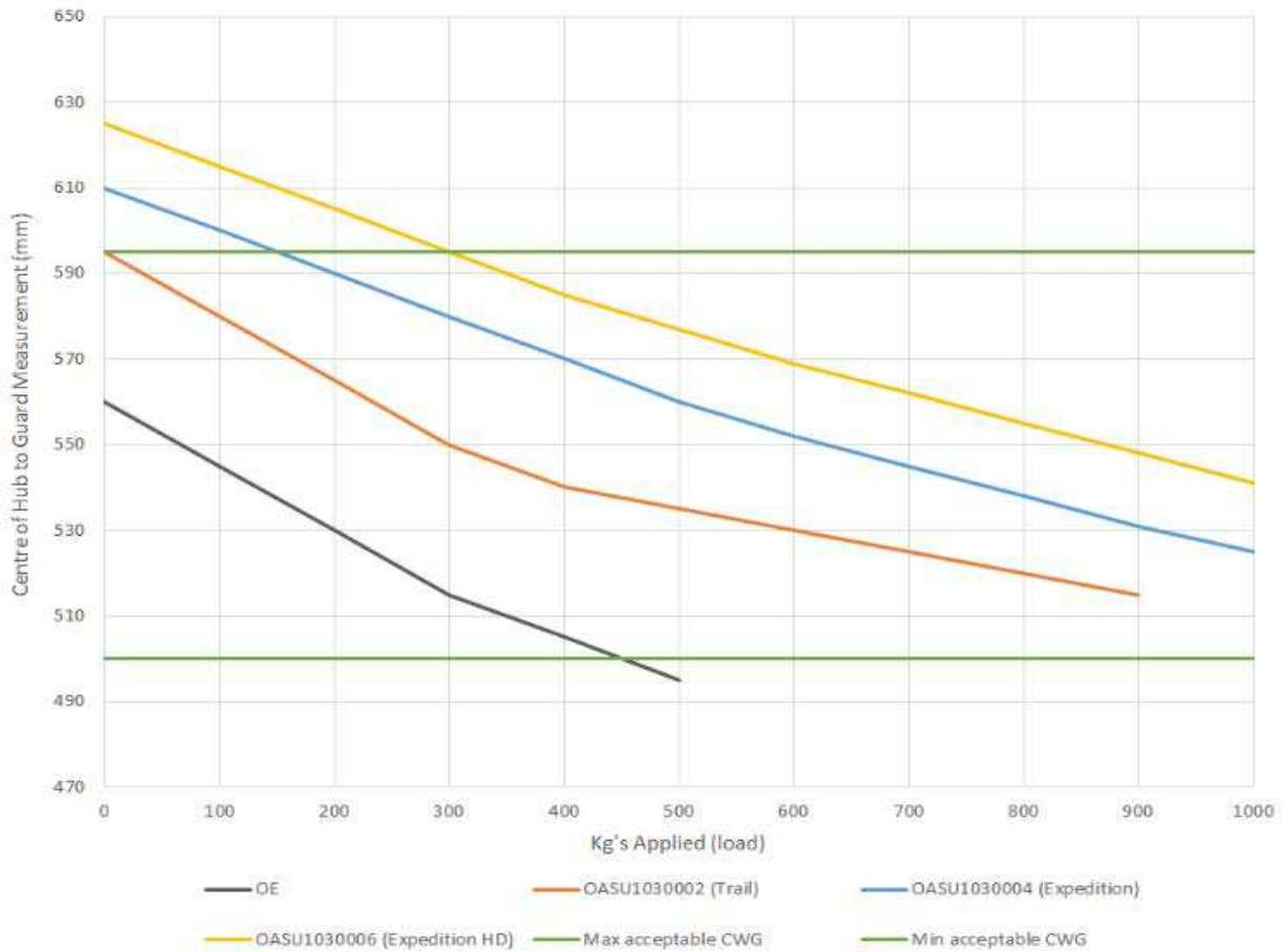
Nissan Navara NP300 Coil Spring Deflection
