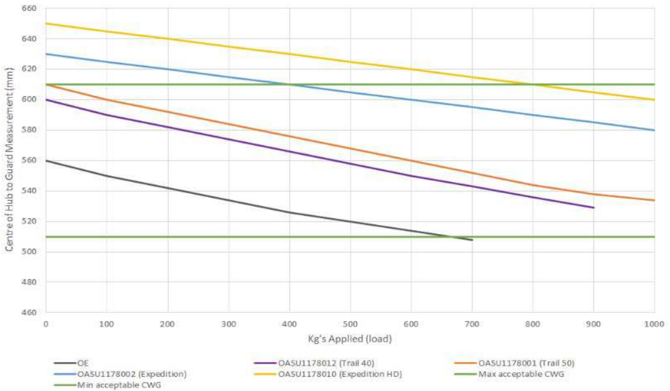
Toyota Landcruiser 78 Series Leaf Spring Deflection
