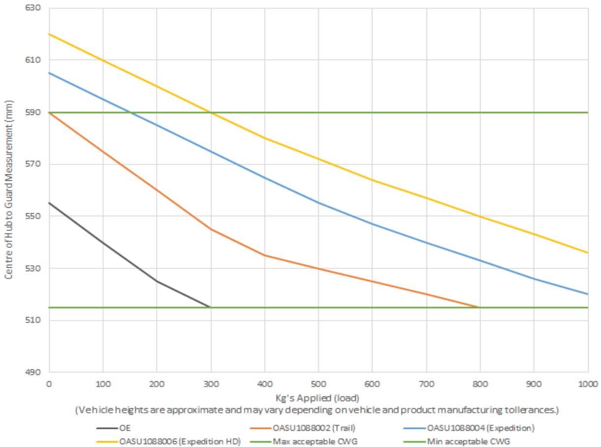
Mercedes Benz X-Class Coil Spring Deflection
