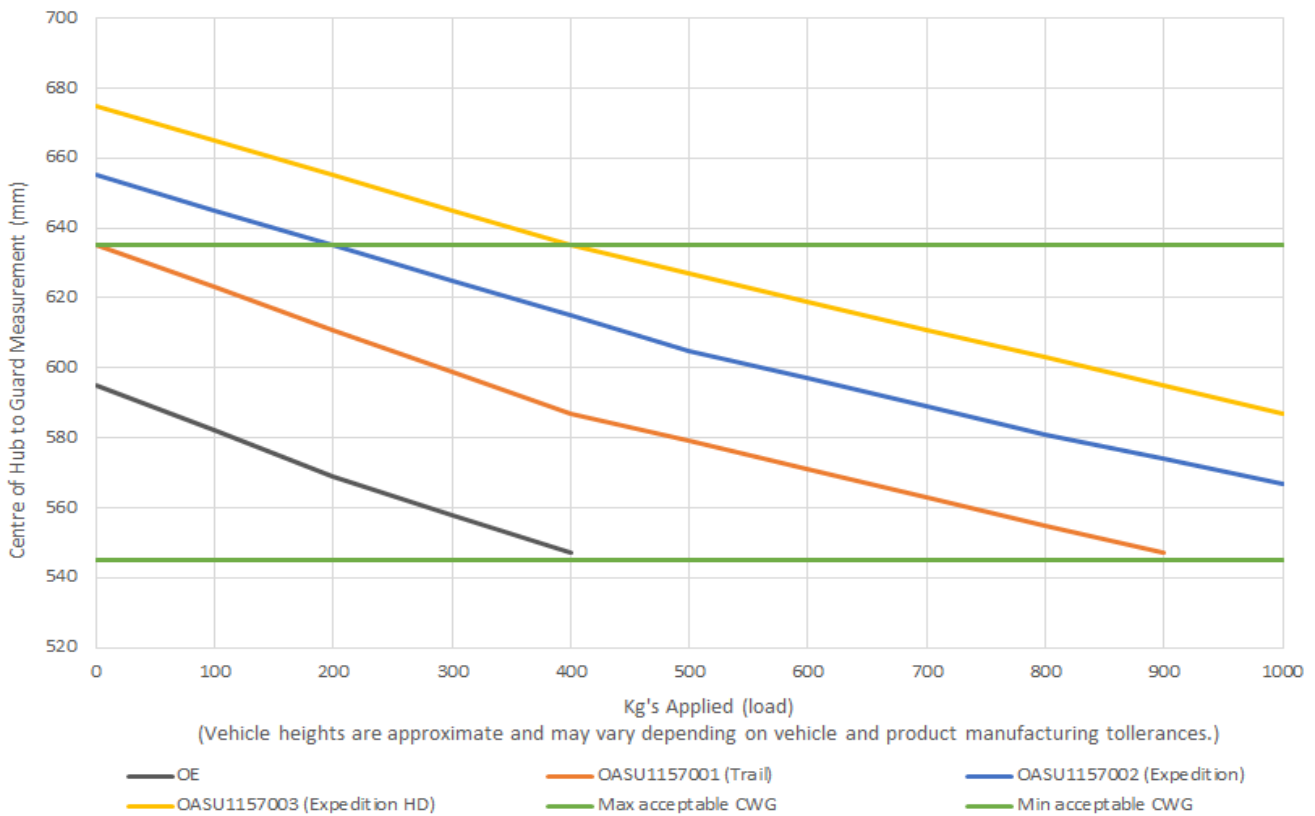
Mitsubishi Triton MQ Leaf Spring Deflection
